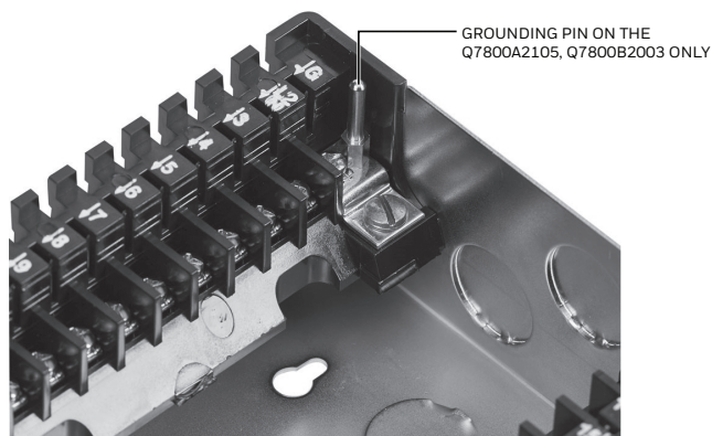
Fig. 2. Series 2000 grounding pin location.
